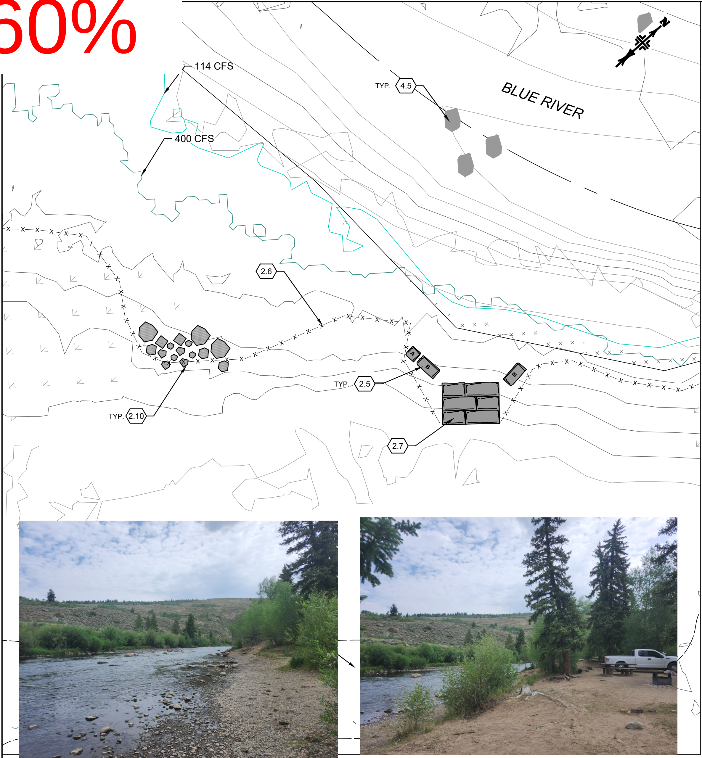
01 LAYOUT AND MATERIALS PLAN
